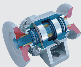
TAPERED BEARINGS AND DUO-CONE TYPE SEALS.
